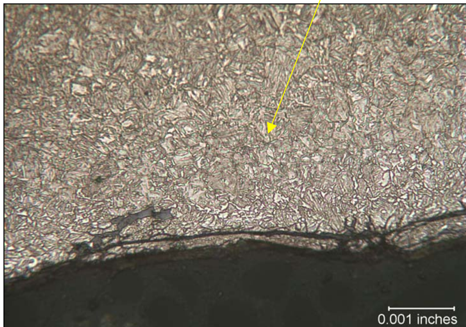
Figure 2: Surface delamination and tears seen at ~200X from process "B" (nital etch).
