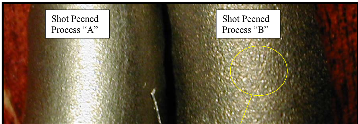
Figure 1: Macro-examination of a spring surface using two different shot peening processes. (~20X)
